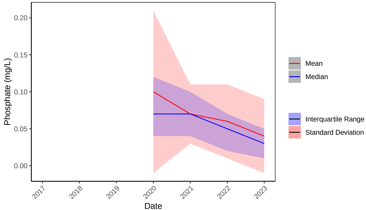
B2 Raceway 1 Phosphate (mg/L) Yearly Statistics
